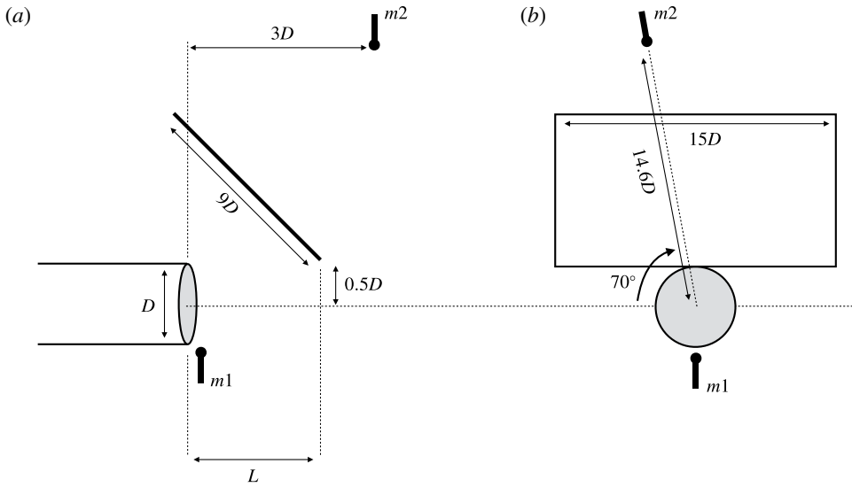
FIGURE 1. Schematic depiction of the experimental set-up. (a) Side view; (b) front view. Points m_1 and m_2 are microphones situated, respectively, in the irrotational, hydrodynamic near field and in the acoustic field.
