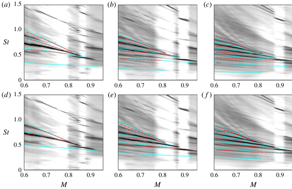
FIGURE 17. Comparison of resonance predictions with experimental data. Solid cyan lines: neutral-mode model; red dash-dotted lines: complex-mode model, with R_1R_2 = 0.002 . Top and bottom: respectively, assumption of in-phase and out-of-phase reflection conditions. From left to right: plate-edge positions L = 2, 3 and 4 .
